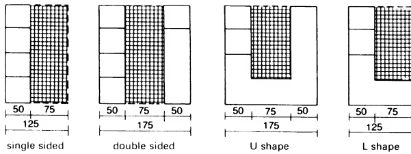
1 Typical larder plans
